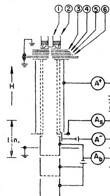
FIG. 3. Electron gun and interaction chamber used for metastable-atom production measurements and elastic scattering. Legend: 1. Cathode, -V_0 ; 2. First accelerating electrode, -V_0+3 ; 3. Second accelerating electrode, -V_0+15 ; 4. Third accelerating electrode, ground; 5. Fourth accelerating electrode, -V_0+(5 \rightarrow 10) ; 6. Fifth accelerating electrode, ground; A + : positive-ion and metastable atom electrometer; A s : scattered electron electrometer; A - : electron-monitoring electrometer; A b : beam current electrometer.
