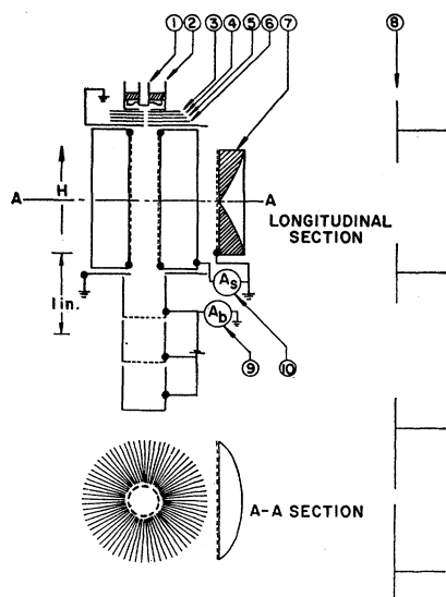
FIG. 2. Electron gun and interaction chamber used for optical intensity measurements and elastic scattering. Legend: 1. Cathode, -V_0 ; 2. First accelerating electrode, -V_0+5 ; 3. Second accelerating electrode, -V_0+15 ; 4. Third accelerating electrode, ground; 5. Fourth accelerating electrode, -V_0+5+\square ; 6. Fifth accelerating voltage, ground; 7. Cylindrical quartz lens; 8. B. and L. 500-mm monochromator; 9. Beam current electrometer; 10. Scattered current electrometer.
